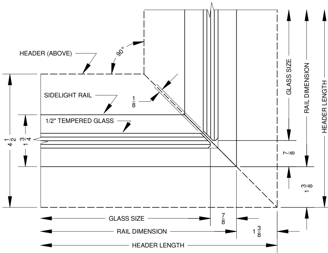
(A) - PLAN DETAIL w/ MITERED GLASS AND MITERED FRAME
