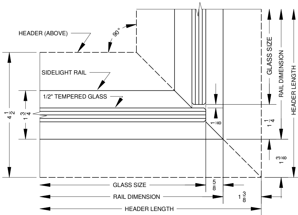
(B) - PLAN DETAIL w/ MITERED FRAME AND OVERLAPPING GLASS
